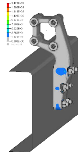
FEM structural and fatigue Analysis
