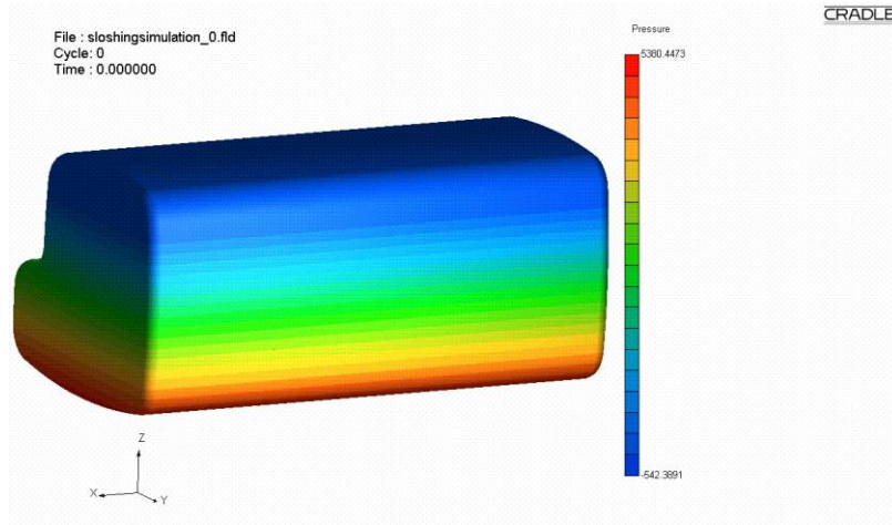
Sloshing Simulation in a diesel tank
